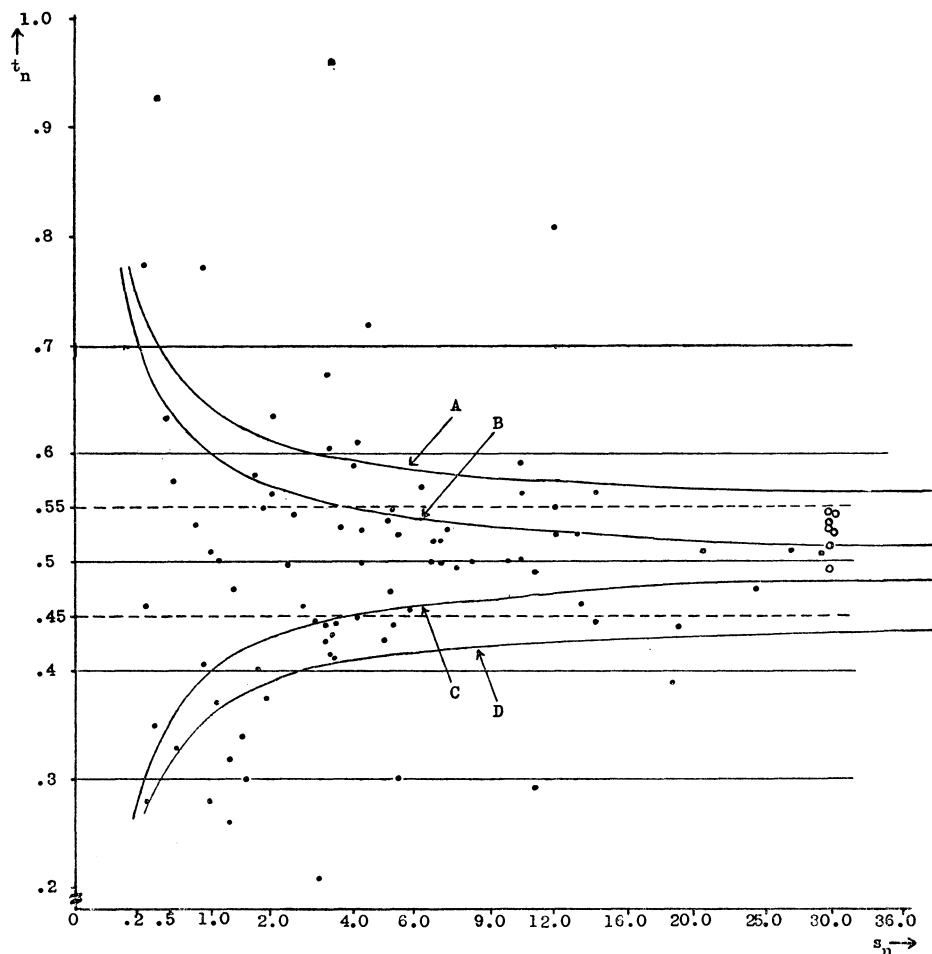
FIG. 5.1. Sample estimates (s_n, t_n) of the parameters (\sigma_n, \tau_n) for 90 function words. Curves B and C show 2 standard error bands for t_n , if \tau_n = .5 . Curve A shows 2 standard error band above \tau_n = .55 . Curve D shows 2 standard error band below \tau_n = .45 .
