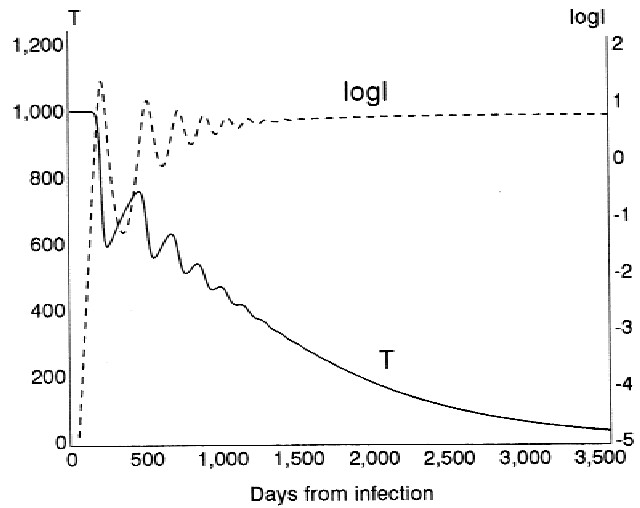
Fig. 3. If viral replicative ability slowly increases model predictions more closely approximate observed patterns. Simulation of model given by equations (1) and (2) with the added component that \phi \cdot \beta increases by a small factor with each replicative cycle. Simulation using Euler approximation with step length 0.1 days. \beta increases by a factor of 1.0002 per infected cell*day. \beta started at a value 0.03 and was 0.83 after 3,650 days (10 years). —, T; ----, logI.
