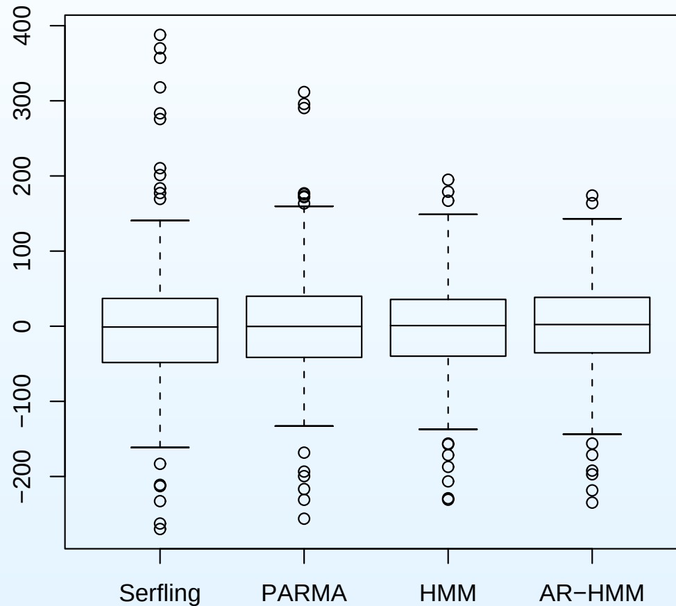
Model residuals
