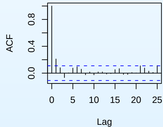
HMM
