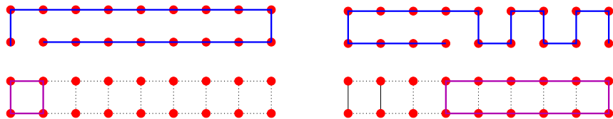
Figure 5: Alternative spanning trees for G and corresponding Steiner cycles.
