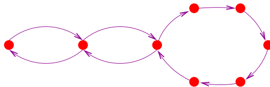
Figure 1: In this (non-simple) cycle C , the number of unique vertices |C| = 8 , but the length of the cycle \ell(C) = 10 .
