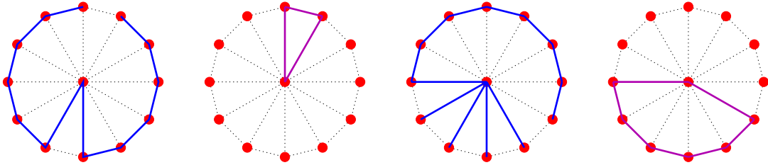
Figure 7: Alternative spanning trees with fewer odd-degree vertices for the wheel graph.
