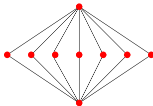
Figure 3: Any spanning tree of this graph has too many leaves to be spanned by a simple cycle. However, note that the solution to the Held-Karp LP relaxation will be |E| = 2n for this graph, certifying that the lower bound is much greater than 4n/3 in this case.
