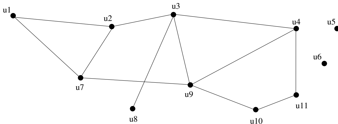
Figure 8: Graph for exercise 23
