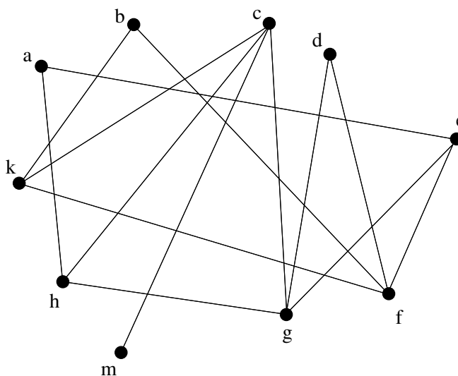
Figure 2: Graph for Exercises 1 and 2
