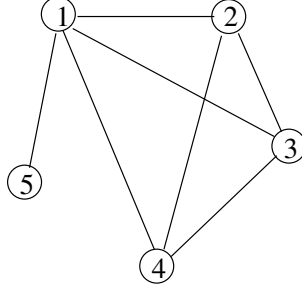
Figure 6: Branch and Bound Example Graph
