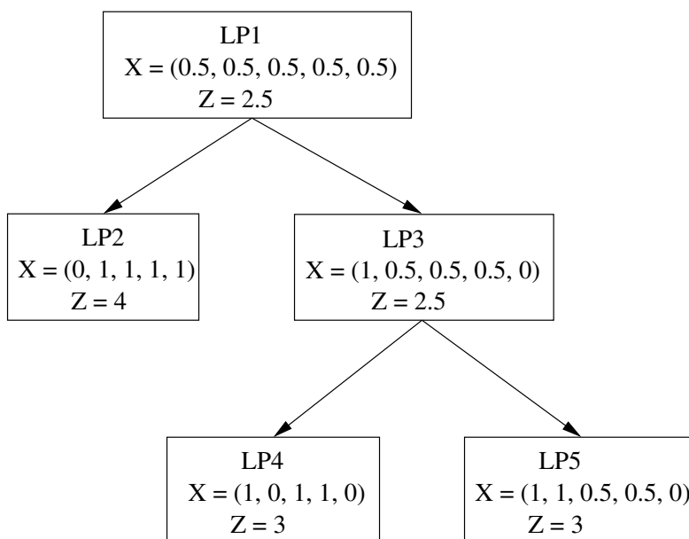
Figure 7: Summary of Branch and Bound IP example
