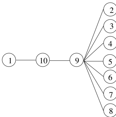
Figure 4: Graph where the approximation is poor
