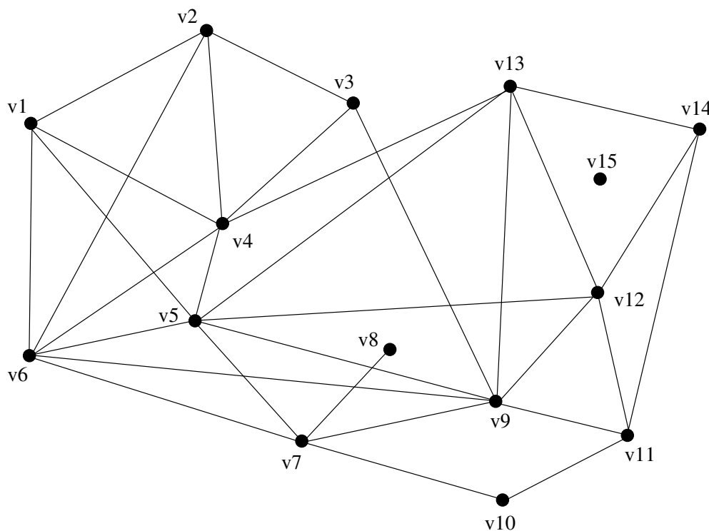
Figure 9: Graph for exercise 24
