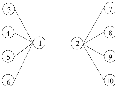
Figure 3: Graph where the approximation is optimal
