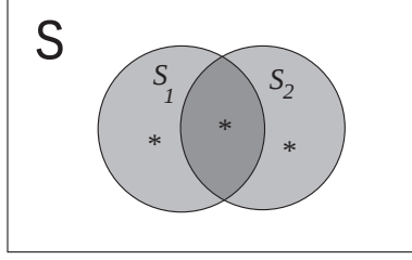
Figure 11: A small non-laminar family.
