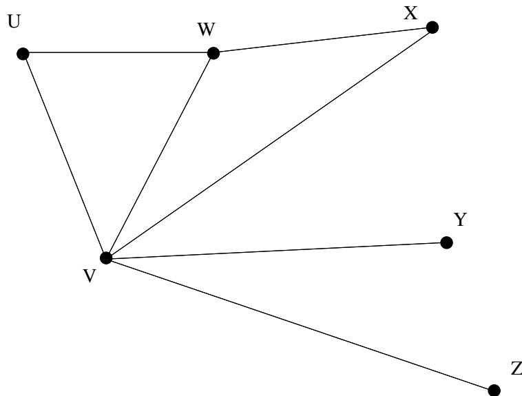
Figure 1: Graph of Size 6
