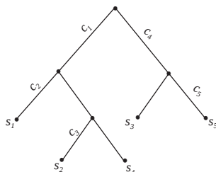
Figure 10: A perfect phylogenetic tree for M_0 .
