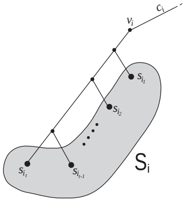
Figure 12: Binary subtree representing S_i .
