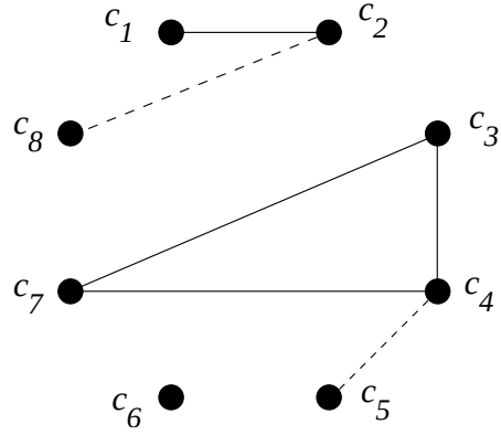
Figure 6.6: The threshold graph G(6) .
